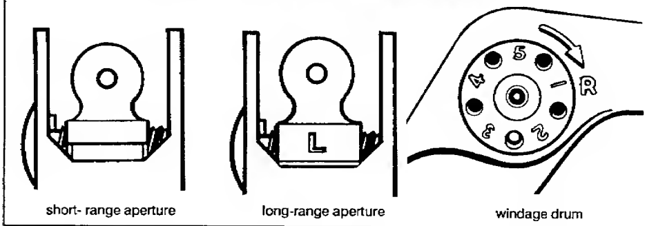
Figure 3-23. M16A1 rear sight apertures and windage drum.
